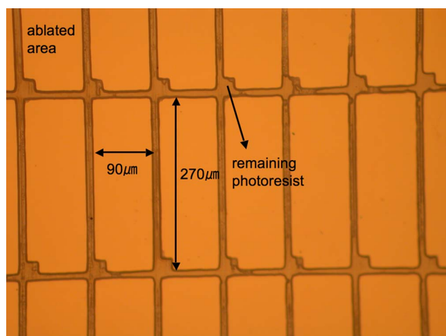
FIG. 2. (Color online) Optical microscope photo of patterns formed in a 2.5\ \mu\text{m} thick photoresist layer on a KrF excimer laser ablation workstation. Using a fluence of 50\ \text{mJ}/\text{cm}^2 at the substrate, the shown patterns were obtained with 30 laser pulses.
