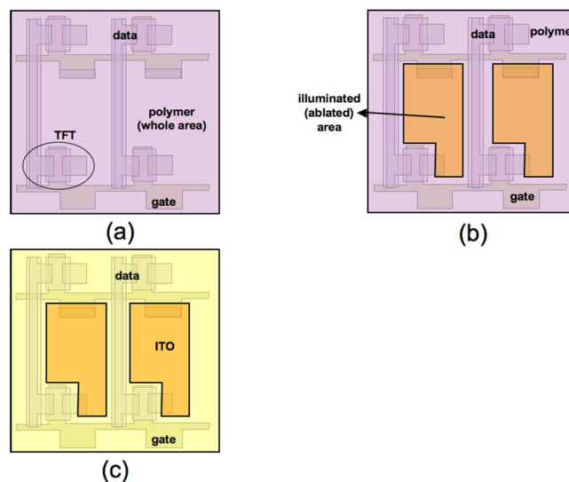
FIG. 4. (Color online) Relationship between the laser illuminated regions, the patterned ITO regions, and the underlying TFT and device regions, illustrating that the laser is never incident on the devices, and therefore this ablation process does not cause any damage.
